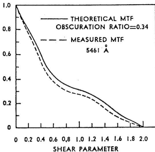
TYPICAL MTF FOR QUESTAR 3 1/2-INCH
